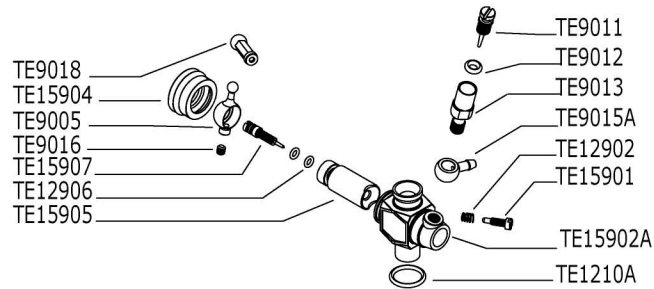
SLIDE CARBURETOR
