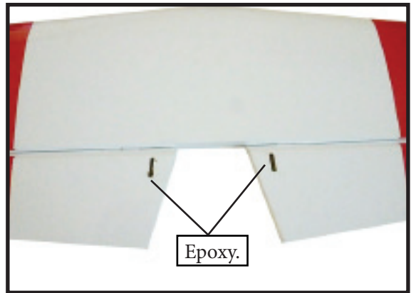
Elevator control horn.
